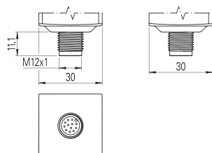
M12-Steckverbinder, axial
