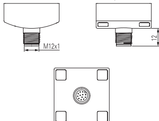
M12-Steckverbinder, axial
