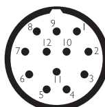
M23-Steckverbinder, 12-polig
