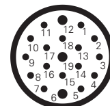
M23 connector, 19-pole
