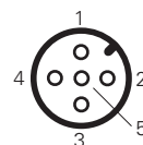
Connector no. 2: Series NG/NS/NX/ST safety switches via VF CY
