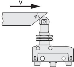
Lever with inverted action (R) - Type 4
