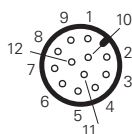
Connectors no. 3, 4, 5 & 6 BN AC3Z... or BN AC4Z... series control device units
