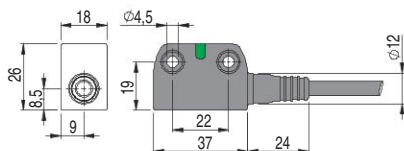
ST G••••M• sensor with M12 connector
